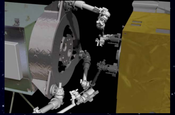
On-orbit servicing
